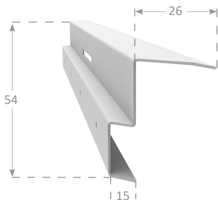
FLANGED EDGE (FEATHERED EDGE) Picture Frame
