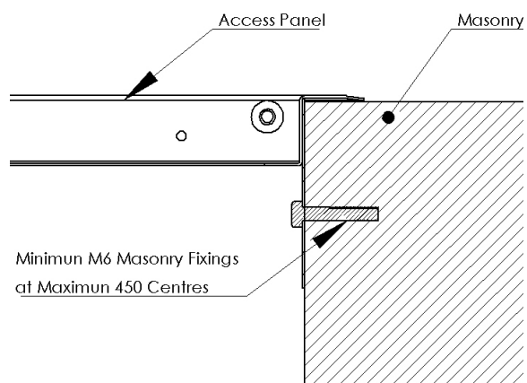
MASONRY Install Profile
