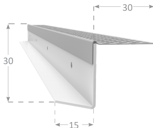
WET WALL (SET BEAD) Concealed Frame
