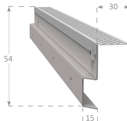
WET WALL (SET BEAD) Concealed Frame
